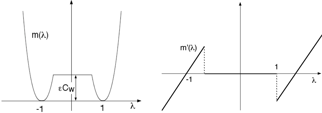
Figure 13: Approximate minimum values for G_\varepsilon^\lambda in Example 9.7
