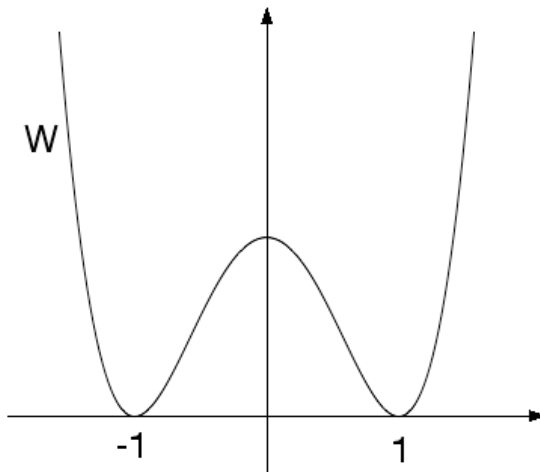
Figure 1: A double-well potential
