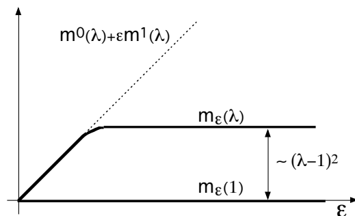
Figure 6: Non-uniformity of the \Gamma -development associated with the nucleation phenomenon
