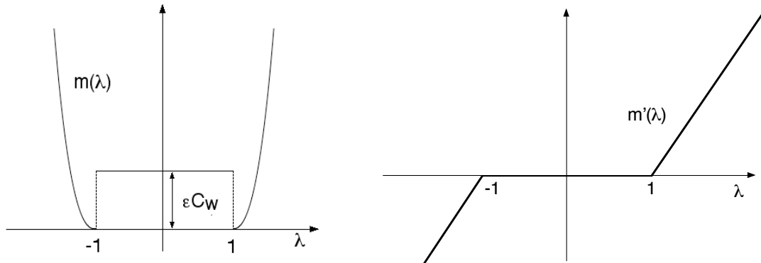
Figure 4: Approximate minimum values by \Gamma -development.
