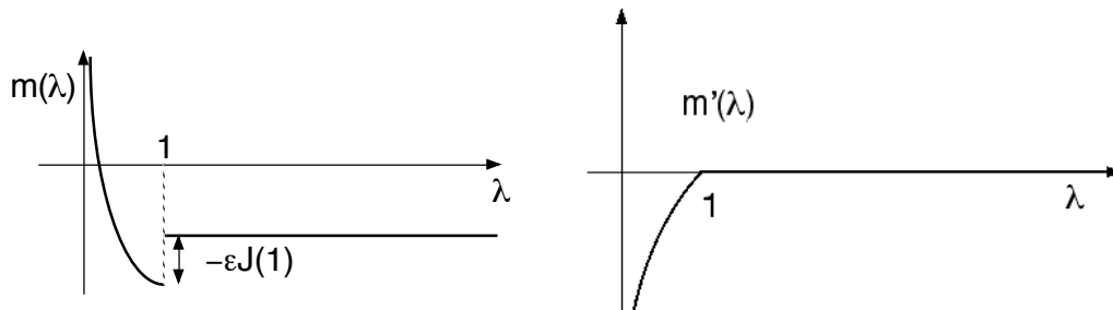
Figure 5: Approximate minimum values by \Gamma -development.
