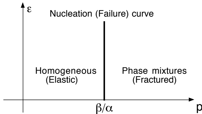
Figure 11: Rectified parameter space in the cases of phase transition and fracture
