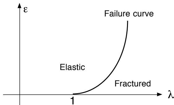
Figure 8: Failure curve in the \varepsilon - \lambda space
