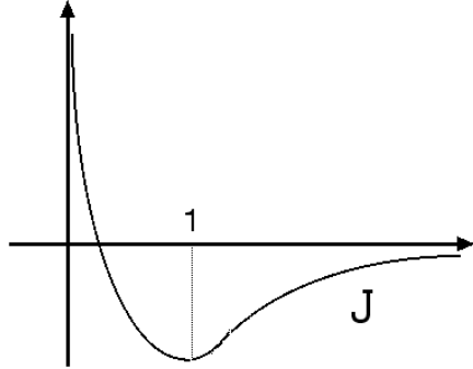
Figure 3: a Lennard-Jones potential.
