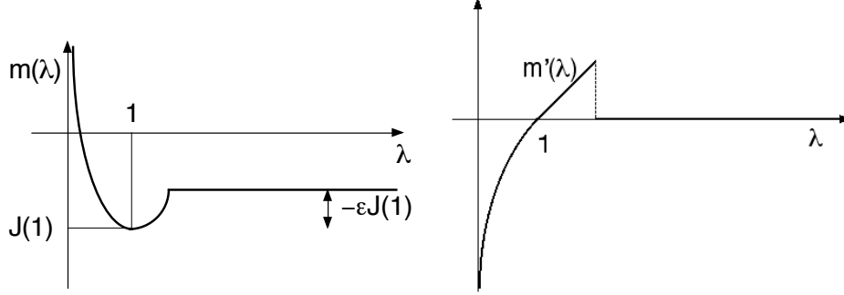
Figure 12: Approximate minimum values for G_\varepsilon^\lambda in Example 9.6
