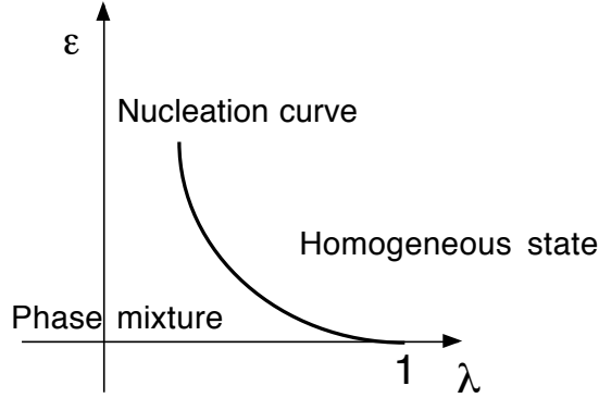
Figure 7: Nucleation curve in the \varepsilon - \lambda space
