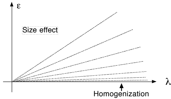
Figure 10: The domain of size effect in the parameter space
