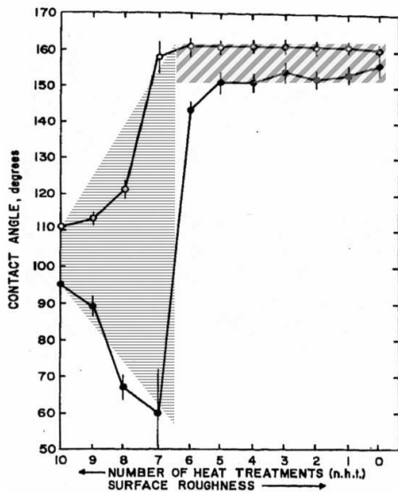
FIGURE 3. Stable contact angles according to our model (shaded regions), superposed on the experimental data from Figure 1.
