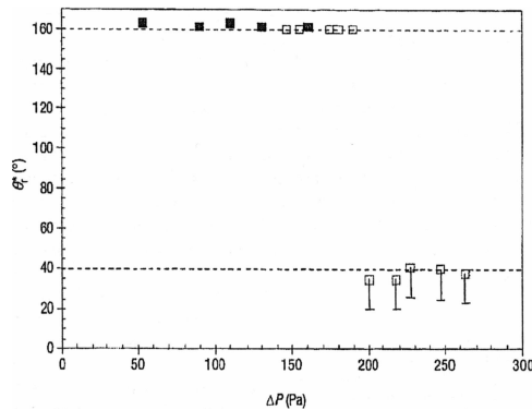
FIGURE 2. Experimental dependence of receding contact angles on the pressure pushing the drop onto the surface. Drops are of CB-type at low pressure and of W-type at high pressure. Reprinted from [LQ] with permission.
